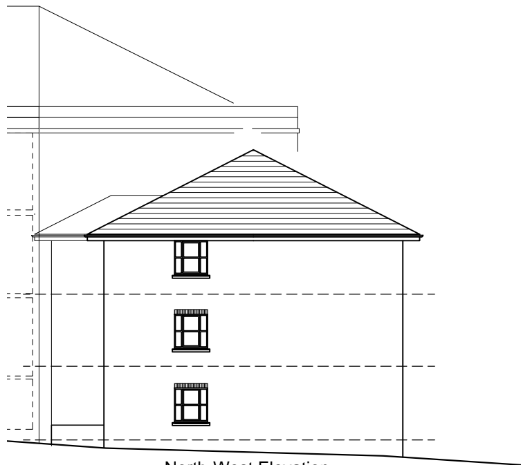
North-West Elevation
